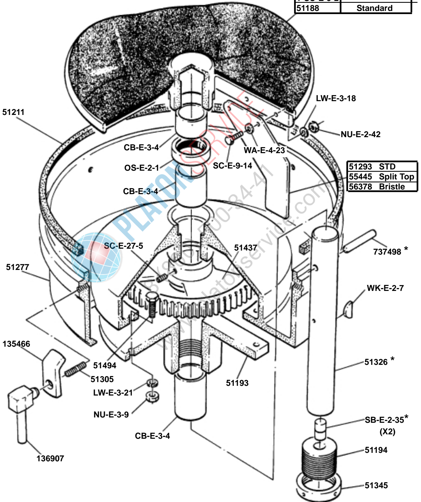
VERTICAL SHAFT ASSEMBLY...142063 Includes Items Marked *
